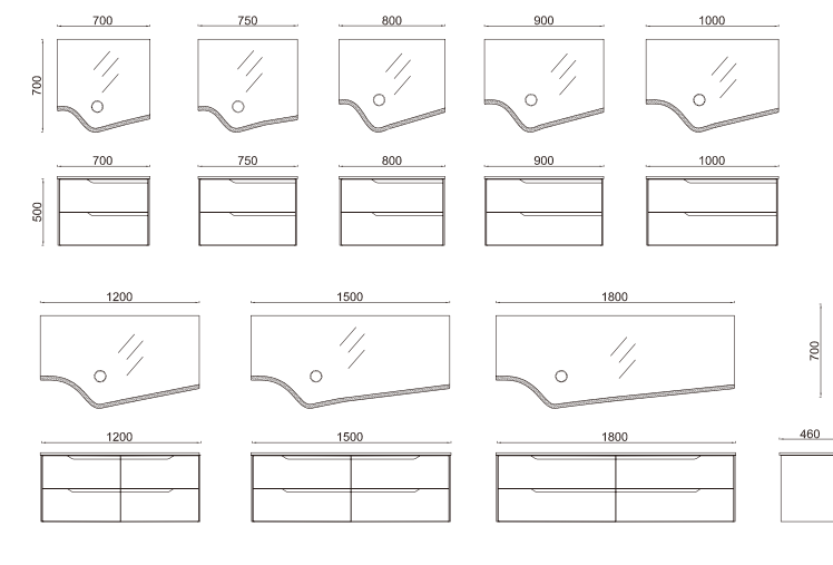
MB-CP87/LS737-1 MDF & Painting
