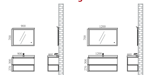
SV1200WH01/S18 Veneer & Painting
