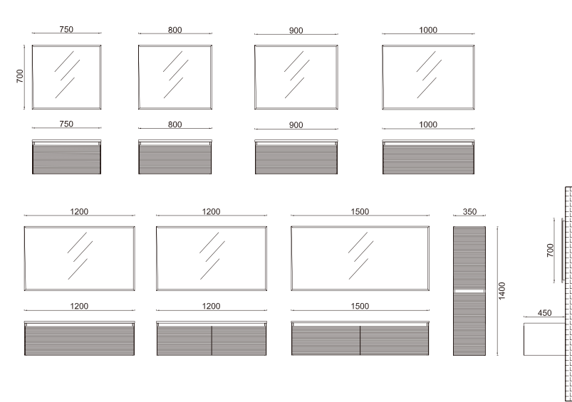
MB-CP85/1200/S40 Plywood & Veneer & Painting
