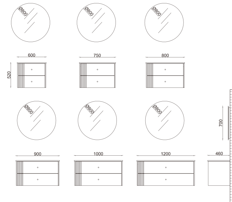
MB-CP86/800/P83 MDF & Painting
