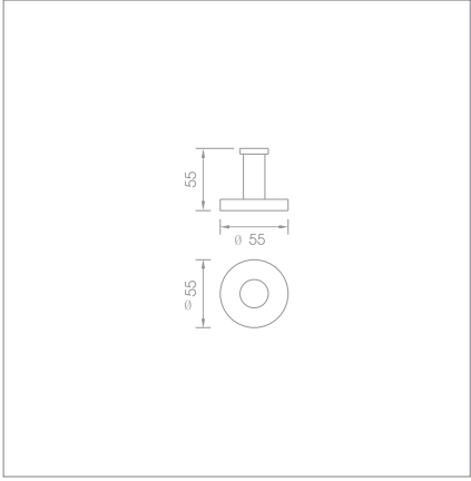
Robe hook Code no.: T2.010 MP T2.010 BP
