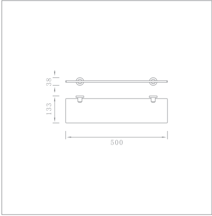
Glass shelf Code no.: 92003
