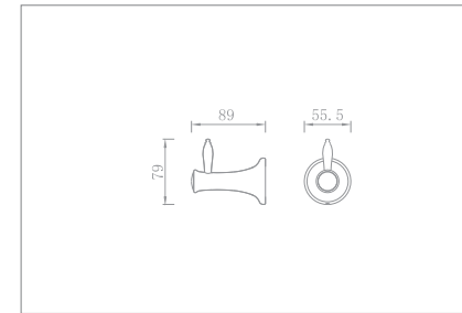
Robe hook Code no.: 56010
