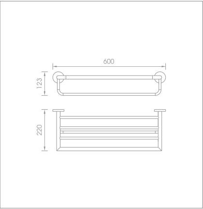
60cm double towel rack Code no.: T2.012 MP T2.012 BP
