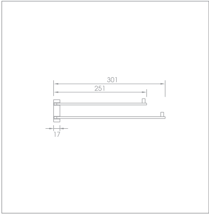
Double swivel towel bar Code no.: F10022
