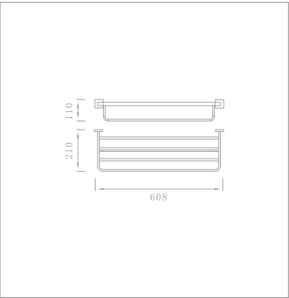
60cm double towel rack Code no.: 95012 Material:Brass Finishing:Chrome
