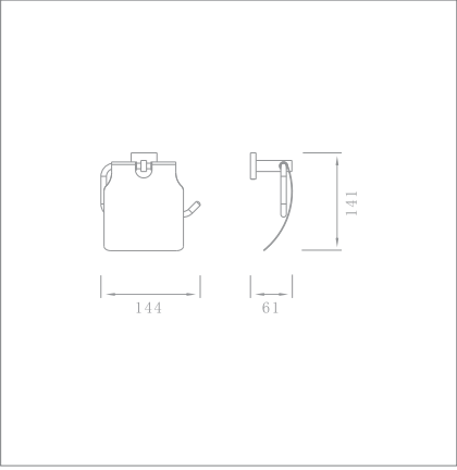
Roll holder with cover Code no.: 95111 Material:Brass+SS304 Finishing: Chrome + Mirror polishing
