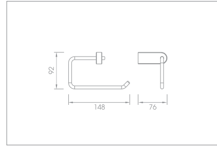
Roll holder Code no.: 87011 MP 87011 BP
