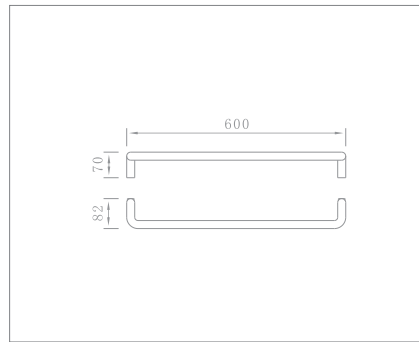
60cm towel bar Code no.: 78001
