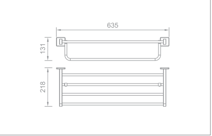
60cm double towel rack Code no.: 87012P MP 87012P BP
