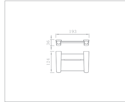
Brass soap dish Code no.: 75107
