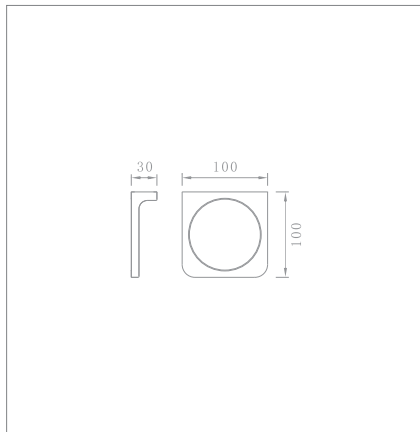
Soap dish holder Code no.: 68107
