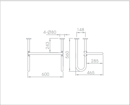
U-type support bar Code no.: 30207 BP Material: SS304 Finishing: Satin
