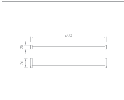
60cm towel bar Code no.: 87001 MP 87001 BP
