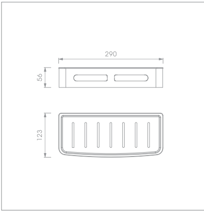
Shower basket Code no.: BS0409 Material: SS304+ABS Finishing: Mirror polishing+White
