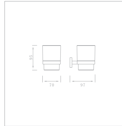
Tumbler holder Code no.: 95006
