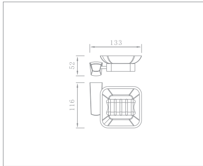
Soap dish Code no.: 75007
