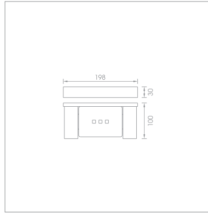
Soap dish holder Code no.: T5.107 MP T5.107 BP
