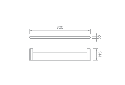
60cm double towel bar Code no.: Q7002
