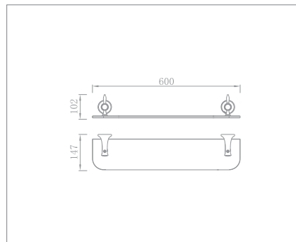
Glass shelf with rail Code no.: 56103 MB
