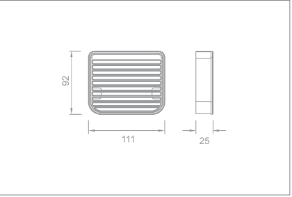
Soap dish holder Code no.: 87007 MP 87007 BP
