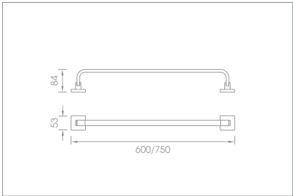
60cm towel bar Code no.: T6.001 MP T6.001 BP
