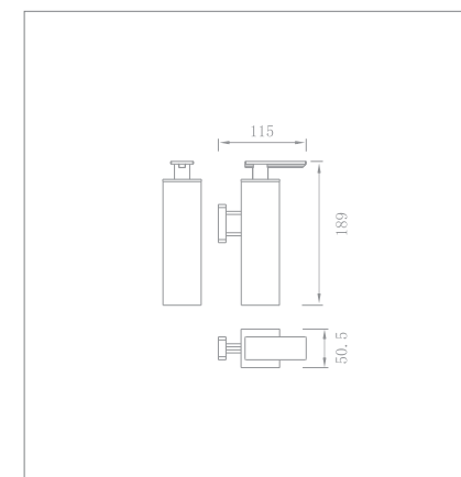
Soap dispenser Code no.: 94016
