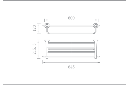
60cm double towel rack Code no.: 56012 MB
