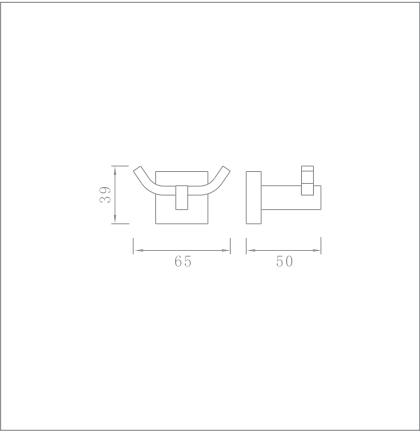
Double robe hook Code no.: 95110 Material:Brass Finishing:Chrome
