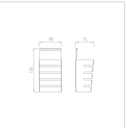
Chopstick basket Code no.: KA2003 Material: Stainless steel Finishing: Black
