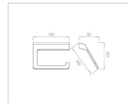
Roll holder Code no.: 61011
