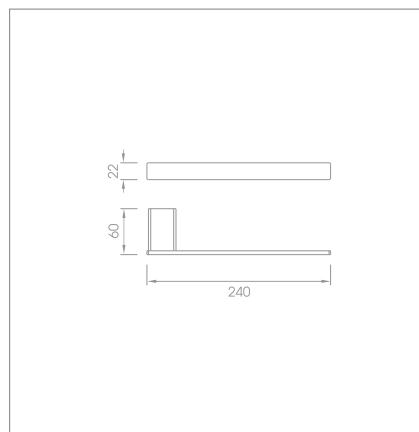
Towel ring Code no.: 71004
