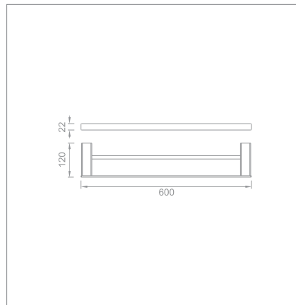
60cm double towel bar Code no.: 71002
