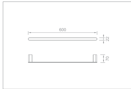
60cm towel bar Code no.: Q7001
