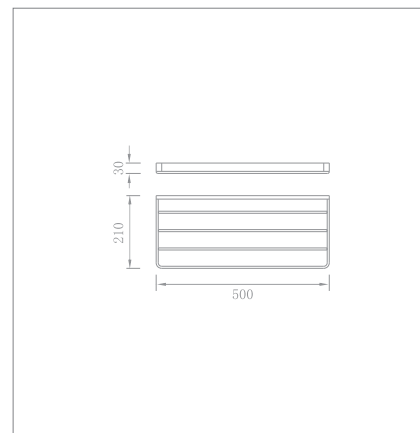
50cm towel rack Code no.: 68012
