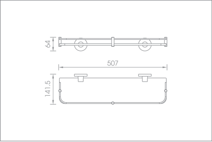
Glass shelf with rail Code no.: T3.203 MP T3.203 BP
