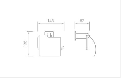
Roll holder with cover Code no.: 87111P MP 87111P BP
