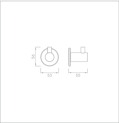
Robe hook Code no.: Q3.010P MP Q3.010P BP
