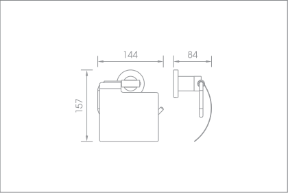
Roll holder with cover Code no.: T3.111 MP T3.111 BP
