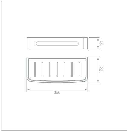
Shower basket Code no.: BS1609 Material: SS304+ABS Finishing: Mirror polishing+White
