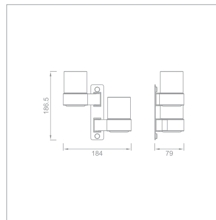
Double tumbler holder Code no.: F7008 MP F7008 BP
