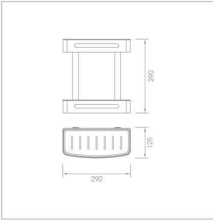
Double shower basket Code no.: BS0639 Material: SS304+ABS Finishing: Mirror polishing+White
