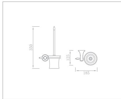
Toilet brush holder Code no.: 56005 MB
