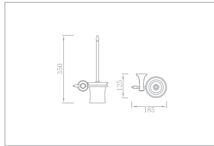
Toilet brush holder Code no.: 56005
