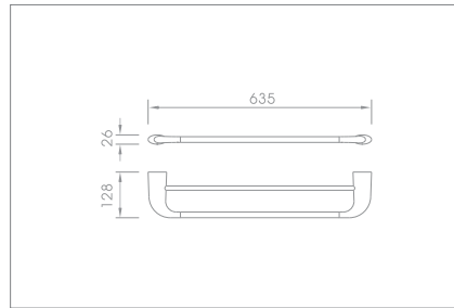
60cm double towel bar Code no.: 52002
