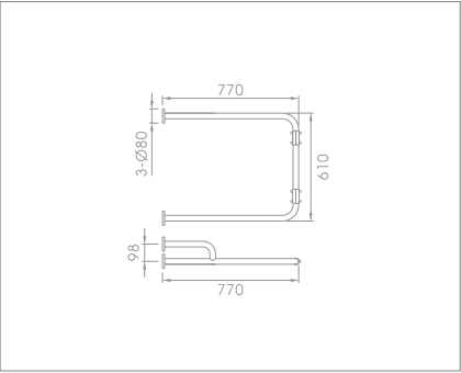
U-type support bar Code no.: 30208 BP Material: SS304 Finishing: Satin
