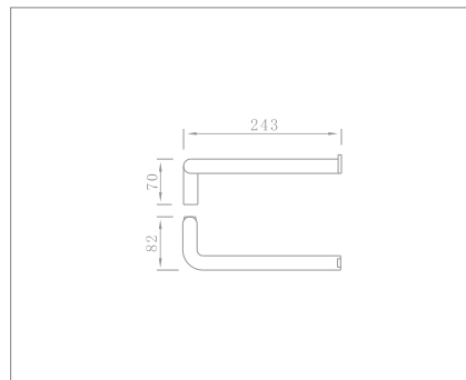
Towel ring Code no.: 78004
