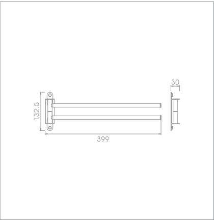
Double swivel bar Code no.: Q3.022P MP Q3.022P BP
