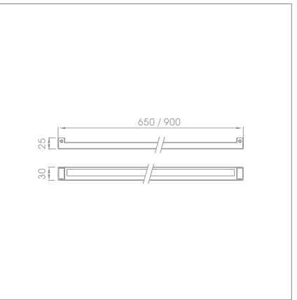
Rail Code no.: KA2006-65 KA2006-90 Material: Stainless steel Finishing: Black
