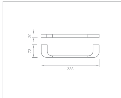
Towel ring Code no.: 70004
