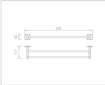
60cm double towel bar Code no.: 87002P MP 87002P BP
