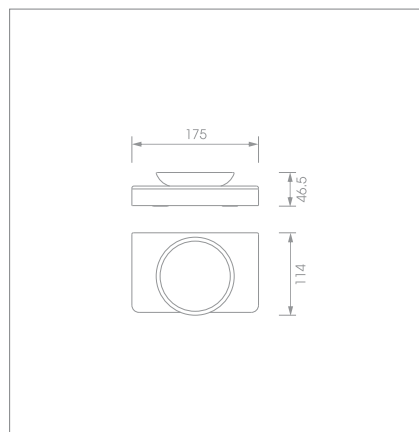
Soap dish holder Code no.: F5007
