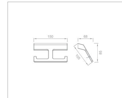
Double robe hook Code no.: 61110
