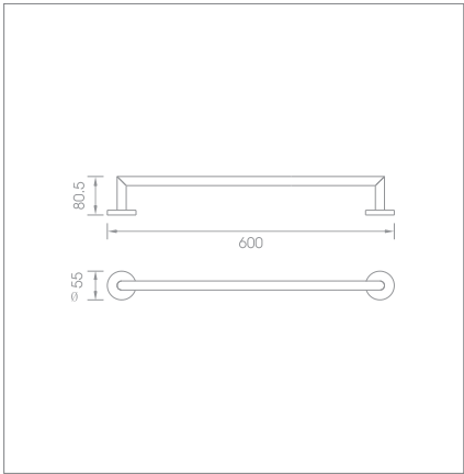
60cm towel bar Code no.: T2.001 MP T2.001 BP
