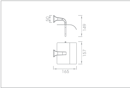
Roll holder with cover Code no.: 88111
