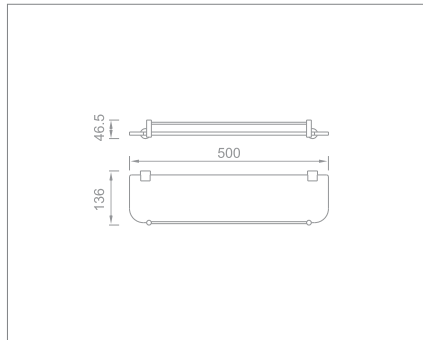
Glass shelf with rail Code no.: Q9.103 MP Q9.103 BP
