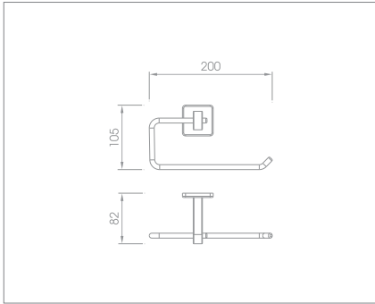
Towel ring Code no.: 87004P MP 87004P BP
