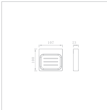
Soap dish holder Code no.: 68207
