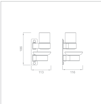
Tumbler holder & Soap dish Code no.: F7108 MB
