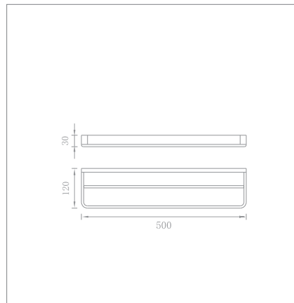
50cm double towel bar Code no.: 68002
