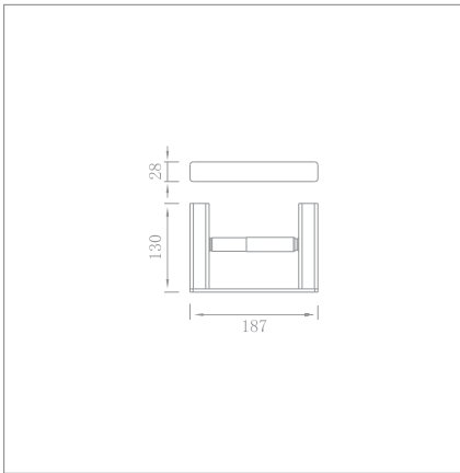
Roll holder Code no.: 72311
