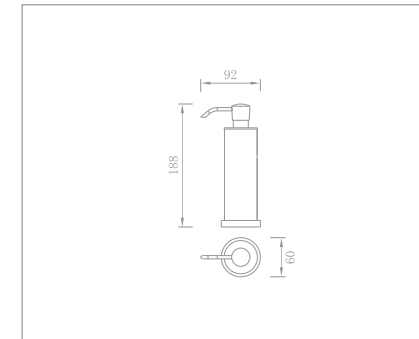
Floor standing soap dispenser Code no.: 20116
