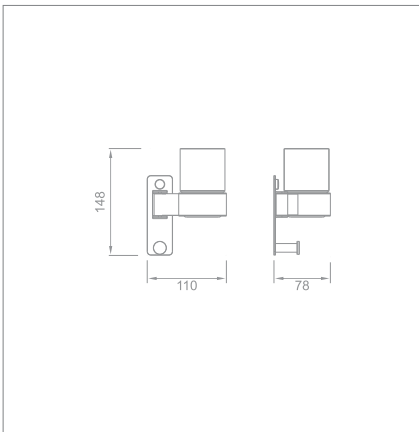
Tumbler holder with hook Code no.: F7006 MB
