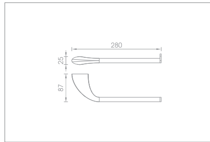
Towel ring Code no.: 52004
