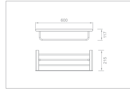
60cm double towel rack Code no.: Q7012
