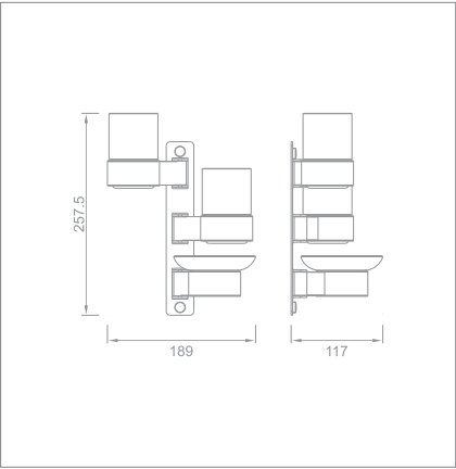
Double tumbler holder & Soap dish Code no.: F7208 MP F7208 BP
