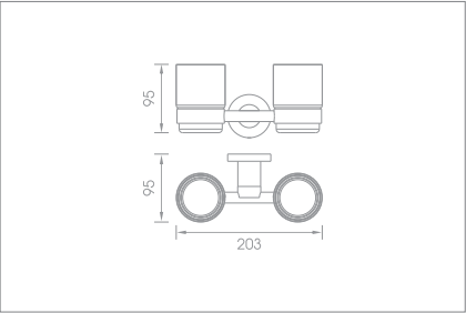
Double tumbler holder Code no.: T2.008 MP T2.008 BP
