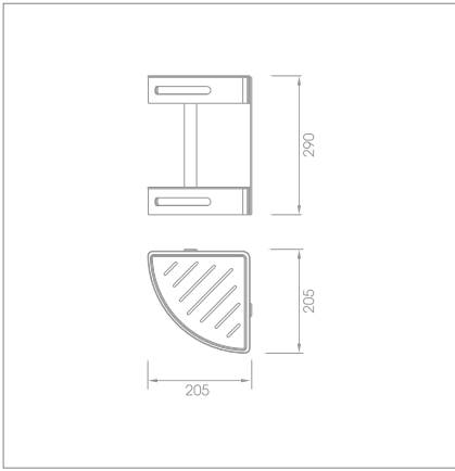
Double corner basket Code no.: BS0739 Material: SS304+ABS Finishing: Mirror polishing+White
