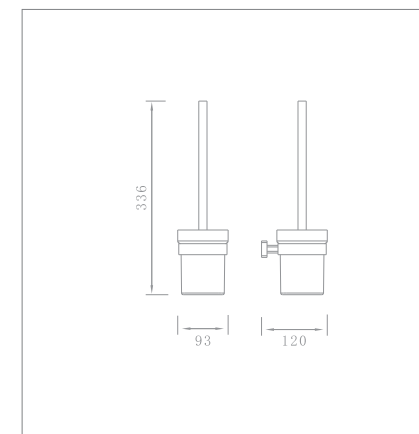
Toilet brush holder Code no.: 94005
