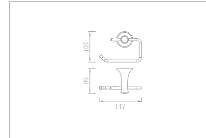
Roll holder Code no.: 56011
