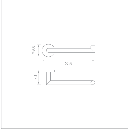
Towel ring Code no.: T2.004 MP T2.004 BP
