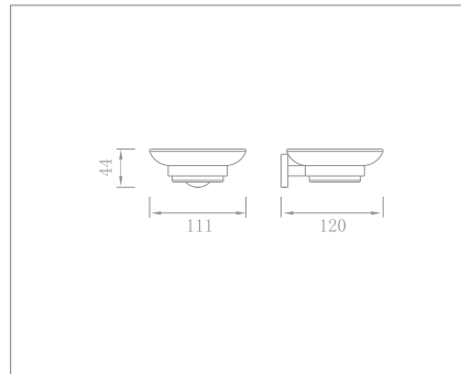
Soap dish holder Code no.: 90307
