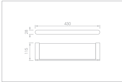
Shelf Code no.: Q5.003 BP
