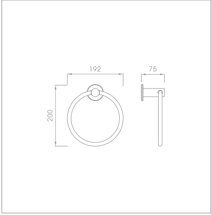
Towel ring Code no.: Q3.104P MP Q3.104P BP
