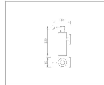
Soap dispenser Code no.: 20016
