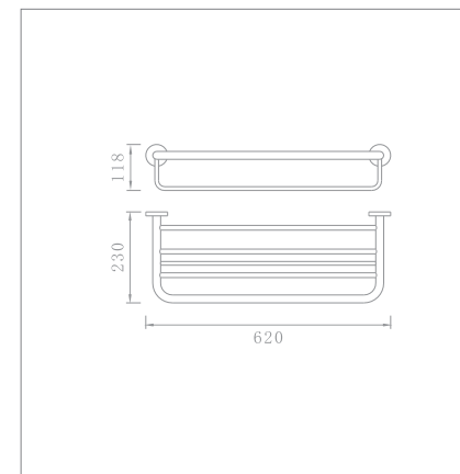
60cm double towel rack Code no.: 92012
