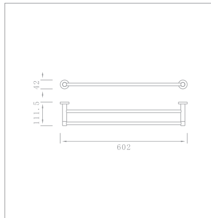
60cm double towel bar Code no.: 90002
