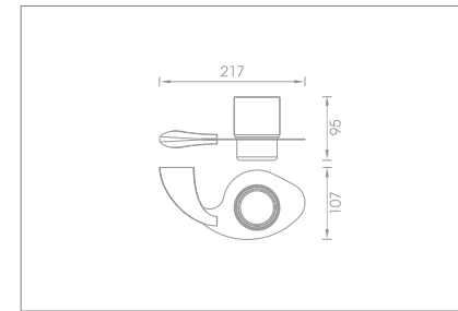
Tumbler holder Code no.: 52006
