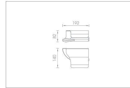
Roll holder with cover Code no.: 52111
