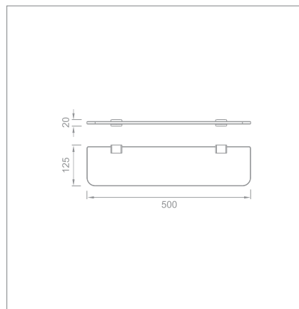
Glass shelf Code no.: 71003
