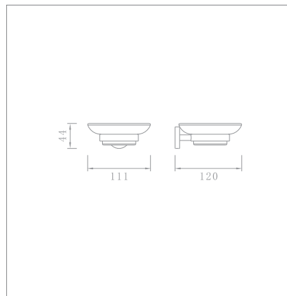
Soap dish holder Code no.: 92007
