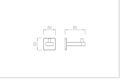
Robe hook Code no.: 87010P MP 87010P BP
