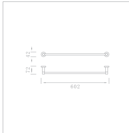
60cm towel bar Code no.: 90001
