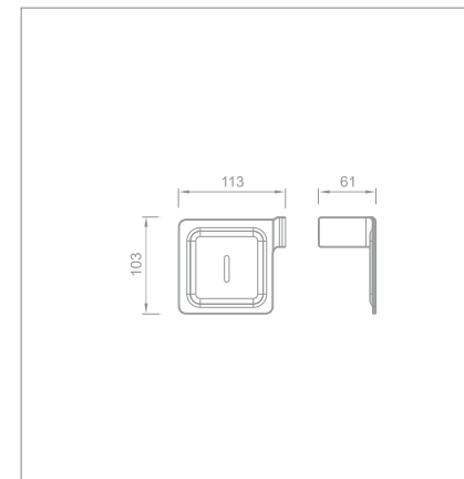
Soap dish holder Code no.: 67107
