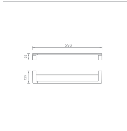
60cm double towel bar Code no.: 67002
