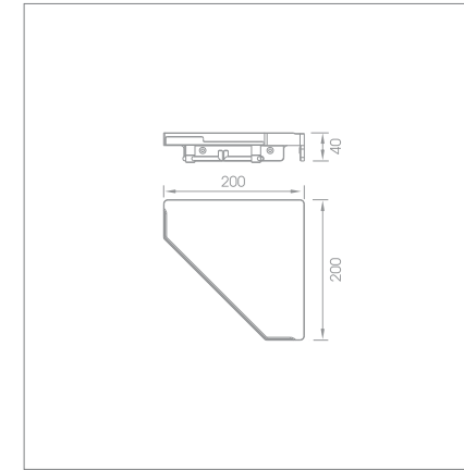
Corner shelf with hook Code no.: F32310 WH
