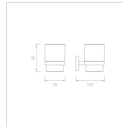
Tumbler holder Code no.: 90306
