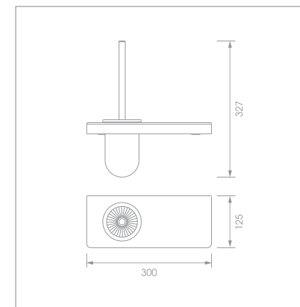
Toilet brush holder & shelf Code no.: F5005
