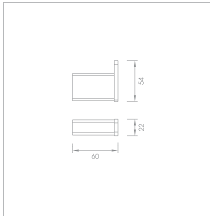
Robe hook Code no.: 71010 MB
