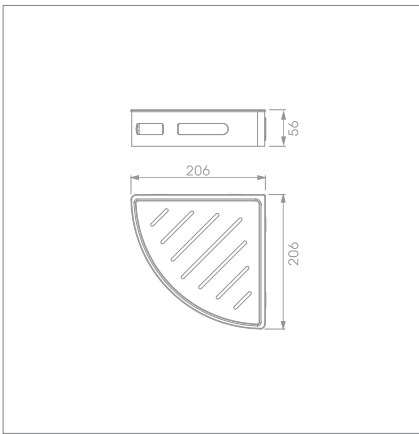
Corner basket Code no.: BS0509 Material: SS304+ABS Finishing: Mirror polishing+White
