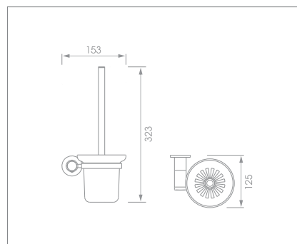
Toilet brush holder Code no.: F4005WC
