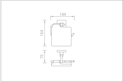
Roll holder with cover Code no.: T6.111 MP T6.111 BP
