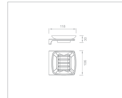
Soap dish Code no.: 61007
