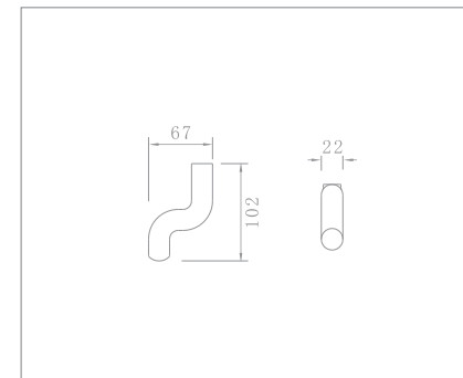
Robe hook Code no.: 78010
