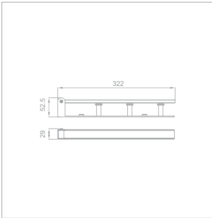
Towel ring with hook Code no.: F7004 MB
