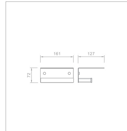
Roll holder with shelf Code no.: 71311 MB
