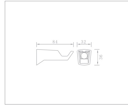
Robe hook Code no.: 75010
