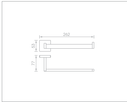
Towel ring Code no.: T7.004 MP T7.004 BP
