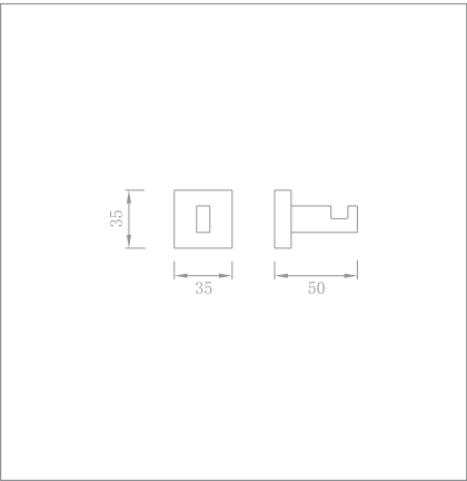
Robe hook Code no.: 95010 Material:Brass Finishing:Chrome
