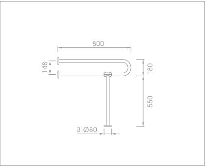
L-type support bar Code no.: 30205 BP Material: 304 Stainless steel Finishing: Satin
