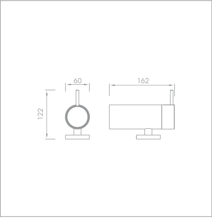
Soap dispenser Code no.: Q3.016P MP Q3.016P BP
