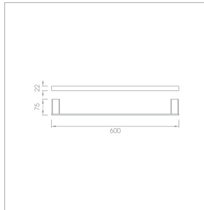
60cm towel bar Code no.: 71001 MB
