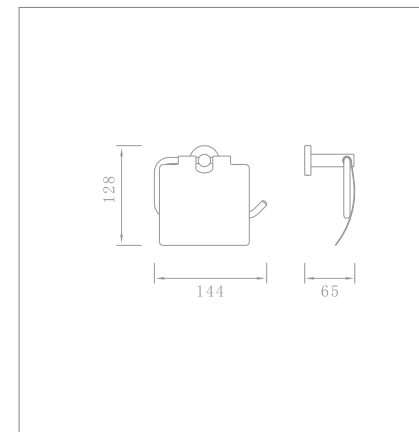
Roll holder with cover Code no.: 92111
