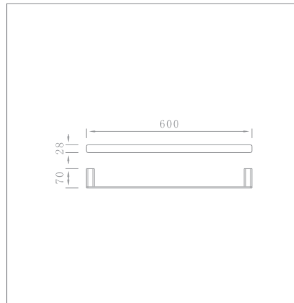
60cm towel bar Code no.: 72001
