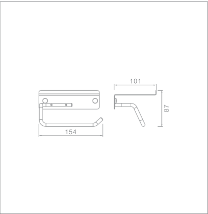
Roll holder with shelf Code no.: T2.411J MP T2.411J BP
