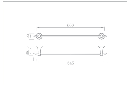
60cm towel bar Code no.: 56001
