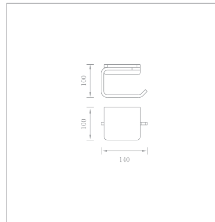
Roll holder with shelf Code no.: 55111
