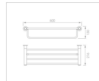
60cm double towel rack Code no.: F4012WC
