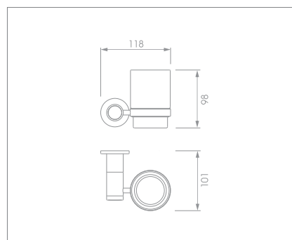
Tumbler holder Code no.: F4006WC
