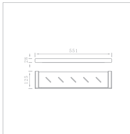
Shelf Code no.: 72003
