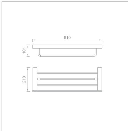
60cm double towel rack Code no.: T5.112 MP T5.112 BP
