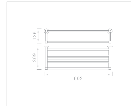
60cm double towel rack Code no.: 90012
