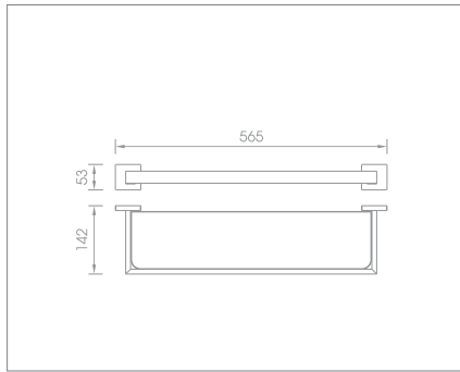
Glass shelf Code no.: T7.003 MP T7.003 BP
