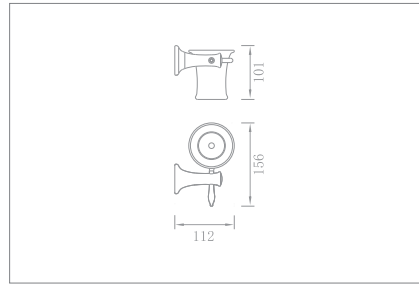
Tumbler holder Code no.: 56006
