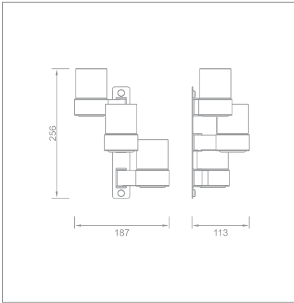
Triple tumbler holder Code no.: F7308 MB
