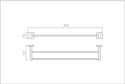
60cm double towel bar Code no.: T9.002 MP T9.002 BP
