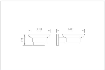
Soap dish holder Code no.: T6.007 MP T6.007 BP
