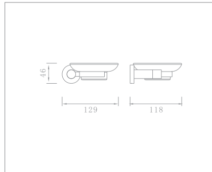
Soap dish holder Code no.: 90007
