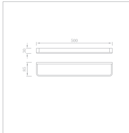
50cm towel bar Code no.: 68001
