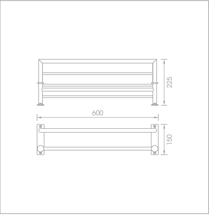
60cm double towel rack Code no.: T2.112 MP T2.112 BP
