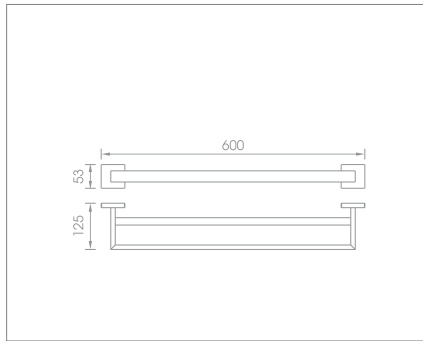
60cm double towel bar Code no.: T7.002 MP T7.002 BP
