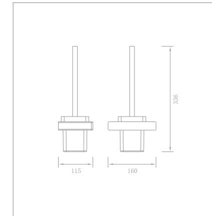
Toilet brush holder Code no.: 72005
