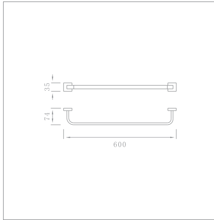
60cm towel bar Code no.: 95001
