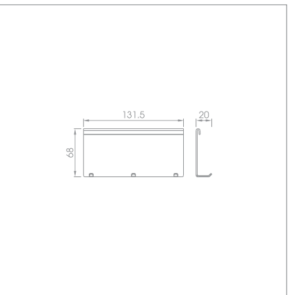
Triple hook Code no.: KA2010 Material: Stainless steel Finishing: Black
