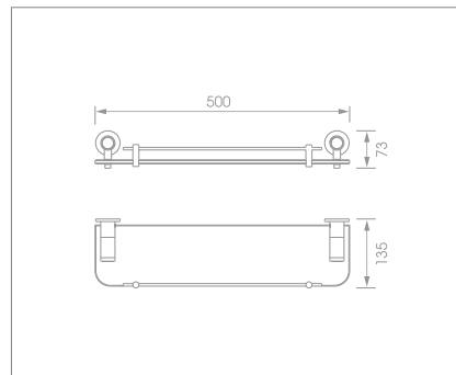
Glass shelf with rail Code no.: F4103WC
