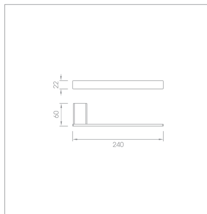
Towel ring Code no.: 71004 MB
