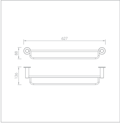
60cm double towel bar Code no.: Q3.102P MP Q3.102P BP
