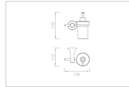
Soap dispenser Code no.: 56016
