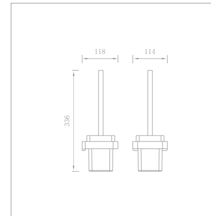
Toilet brush holder Code no.: 68005
