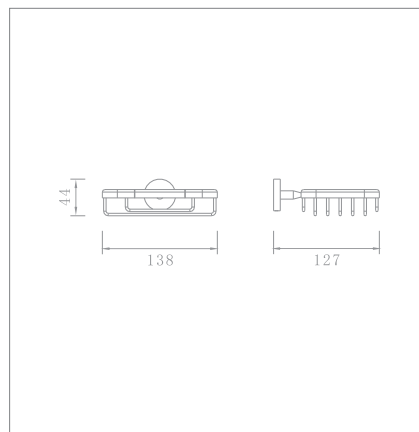
Soap basket Code no.: 92009
