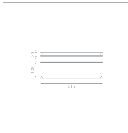
Shelf Code no.: 68003
