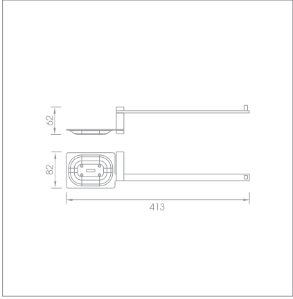
Soap dish holder & Towel ring Code no.: F11704
