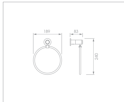
Towel ring Code no.: F4004WC
