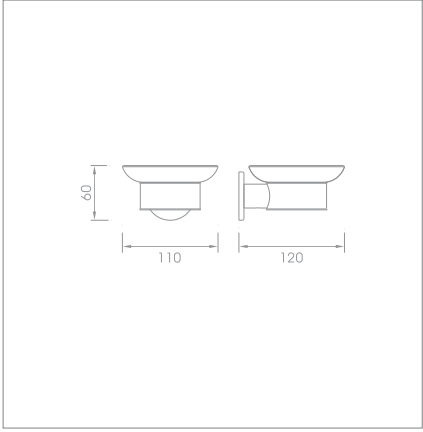
Soap dish holder Code no.: Q3.007P MP Q3.007P BP
