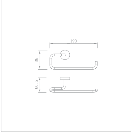
Towel ring Code no.: 92104
