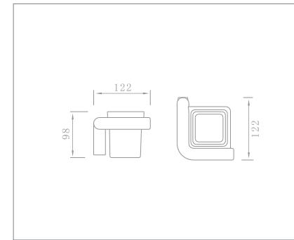
Tumbler holder Code no.: 78006
