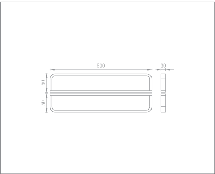
Handle for shower enclosure Code no.: 68018 Material: Brass Finishing: Chrome
