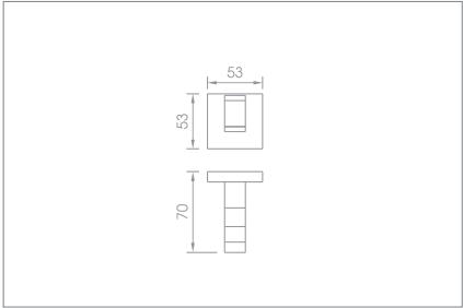
Robe hook Code no.: T6.010 MP T6.010 BP
