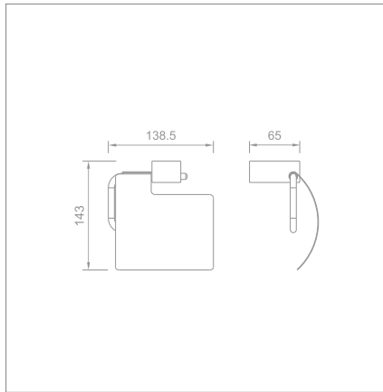
Roll holder with cover Code no.: T5.111 MP T5.111 BP
