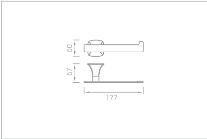
Roll holder Code no.: 88011
