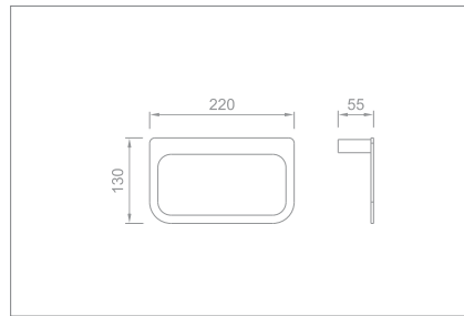
Towel ring Code no.: Q7004
