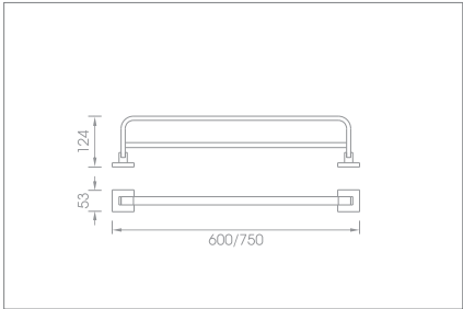
60cm double towel bar Code no.: T6.002 MP T6.002 BP
