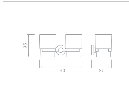
Double tumbler holder Code no.: 90008
