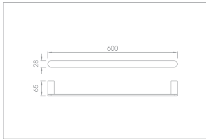
60cm towel bar Code no.: Q5.001 BP
