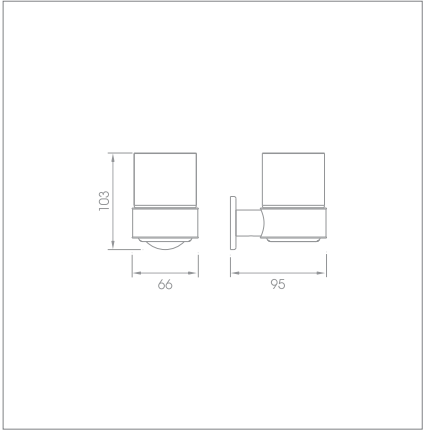
Tumbler holder Code no.: Q3.006P MP Q3.006P BP
