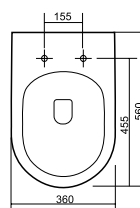
TOP VIEW
